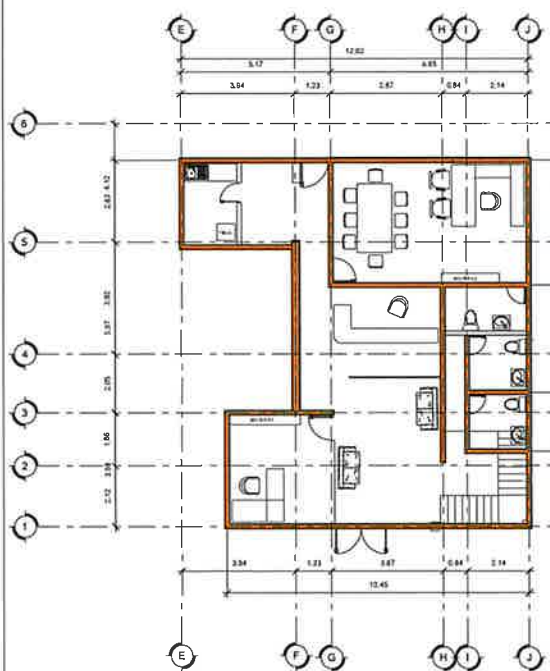
1 Planta General PB 1 : 75
